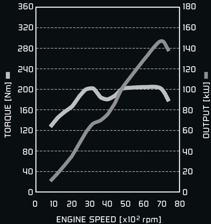
Power & Torque Performance
